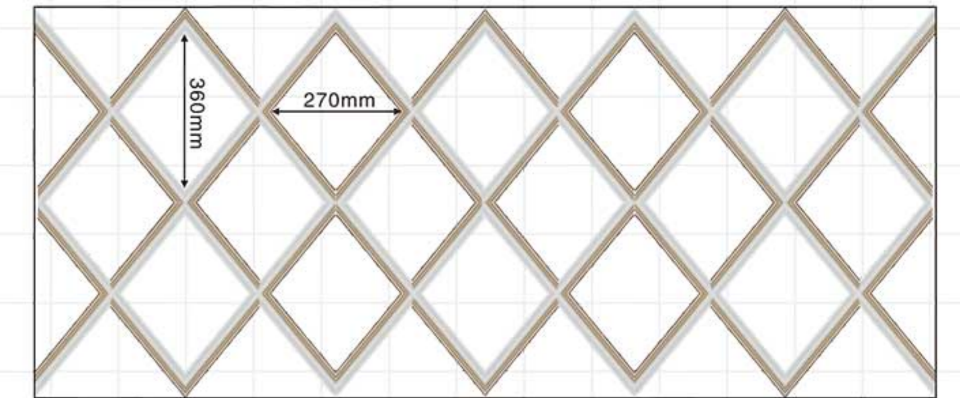
M-7409 D:460x300x15mm
