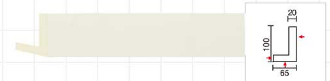
GD-85095-65 L:2400mm
