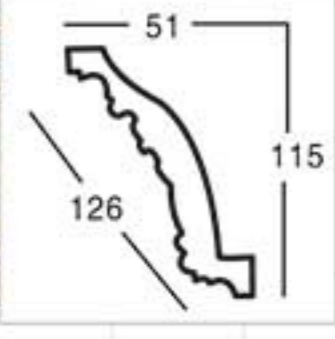
GA-81113 L:2400mm Breadth:126mm Pattern:1230mm
