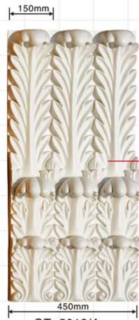
GT-5012/A 955x450x160mm
