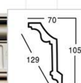
GA-81018-105 L:2400mm Breadth:129mm Pattern:122mm
