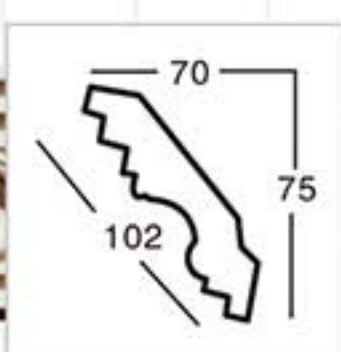
GA-81021 L:2400mm Breadth:102mm Pattern:300mm
