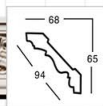
GA-81013 L:2400mm Breadth:94mm Pattern:100mm
