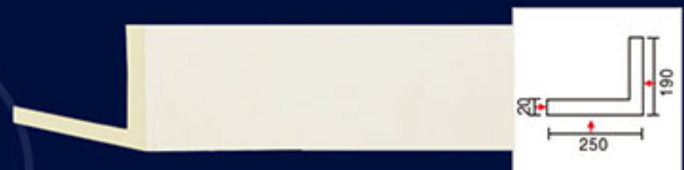
GD-85095-250 L:2400mm
