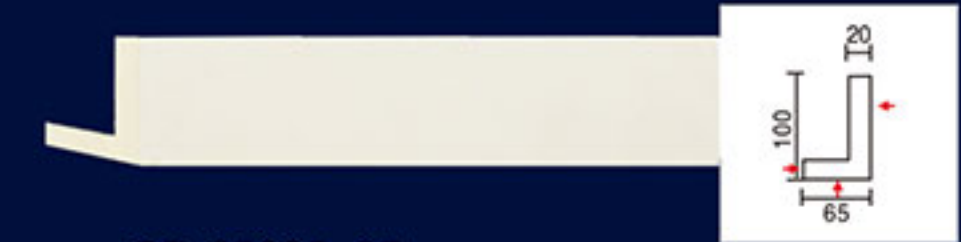
GD-85095-65 L:2400mm
