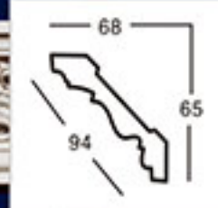
GA-81013 L:2400mm Breadth:94mm Pattern:100mm
