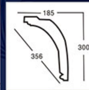
GA-81169 L:2400mm Breadth:356mm Pattern:122mm
