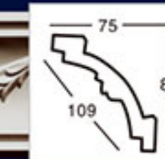
GA-81024 L:2400mm Breadth:109mm Pattern:204mm
