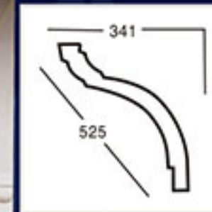
GA-81173 L:2100mm Breadth:525mm Pattern:60mm
