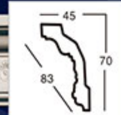
GA-81018-70 L:2400mm Breadth:83mm Pattern:45mm
