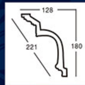
GA-81160 L:2400mm Breadth:221mm Pattern:486mm
