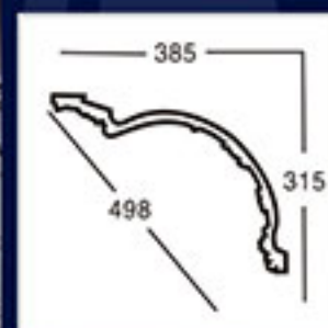
GA-81170 L:2400mm Breadth:498mm Pattern:244mm
