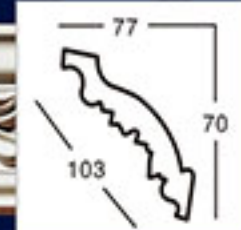
GA-81020 L:2400mm Breadth:103mm Pattern:240mm
