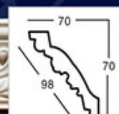
GA-81017 L:2400mm Breadth:98mm Pattern:200mm
