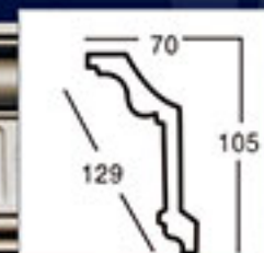
GA-81018-105 L:2400mm Breadth:129mm Pattern:122mm
