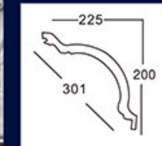
GA-81175 L:2400mm Breadth:301mm Pattern:490mm
