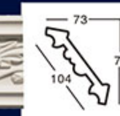
GA-81025 L:2400mm Breadth:104mm Pattern:205mm
