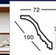
GA-81023 L:2400mm Breadth:100mm Pattern:164mm
