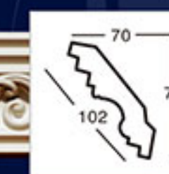
GA-81021 L:2400mm Breadth:102mm Pattern:300mm
