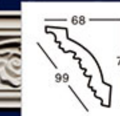
GA-81022-70 L:2400mm Breadth:99mm Pattern:240mm
